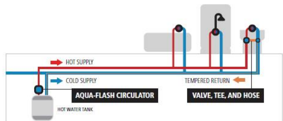
Install pump with timer, 10 ft. cord, on top of water heater
